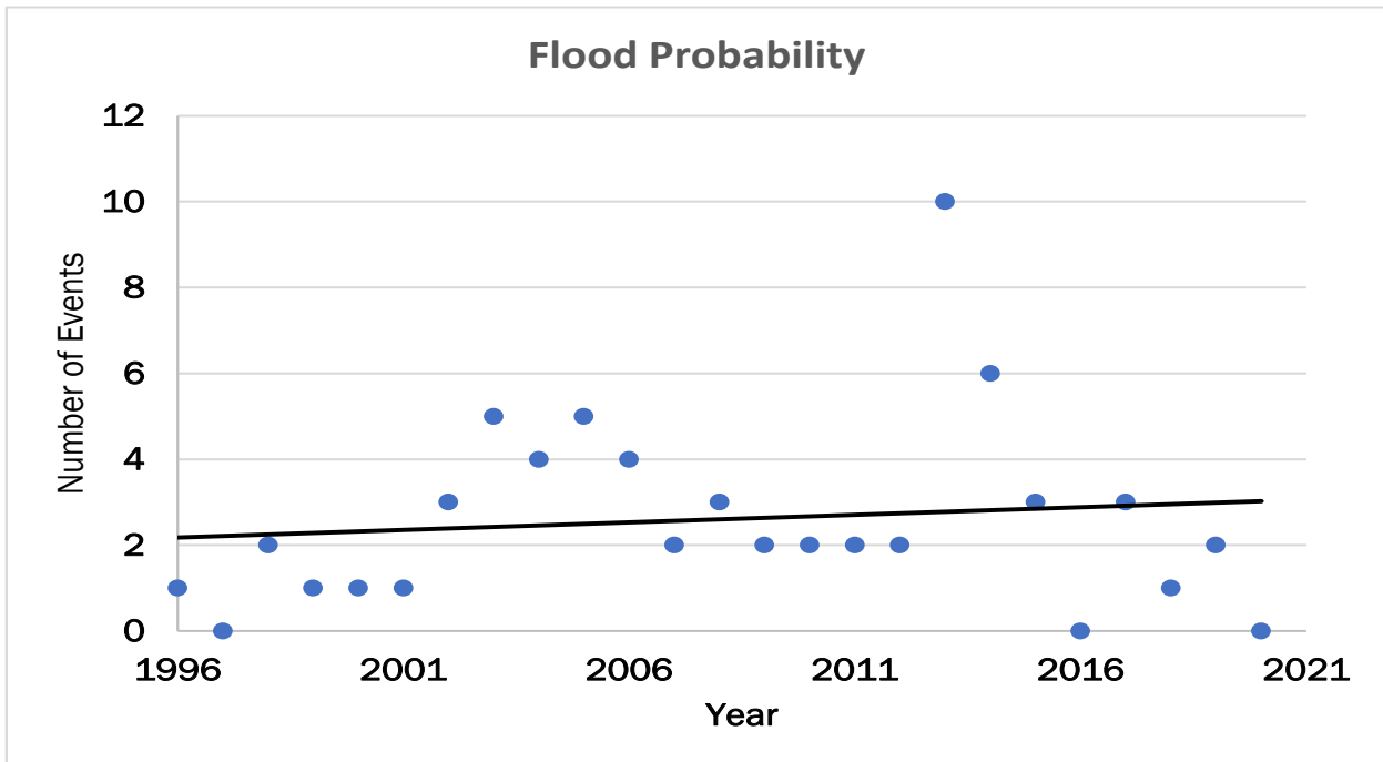
Figure 4.5.2 Flood Probability
