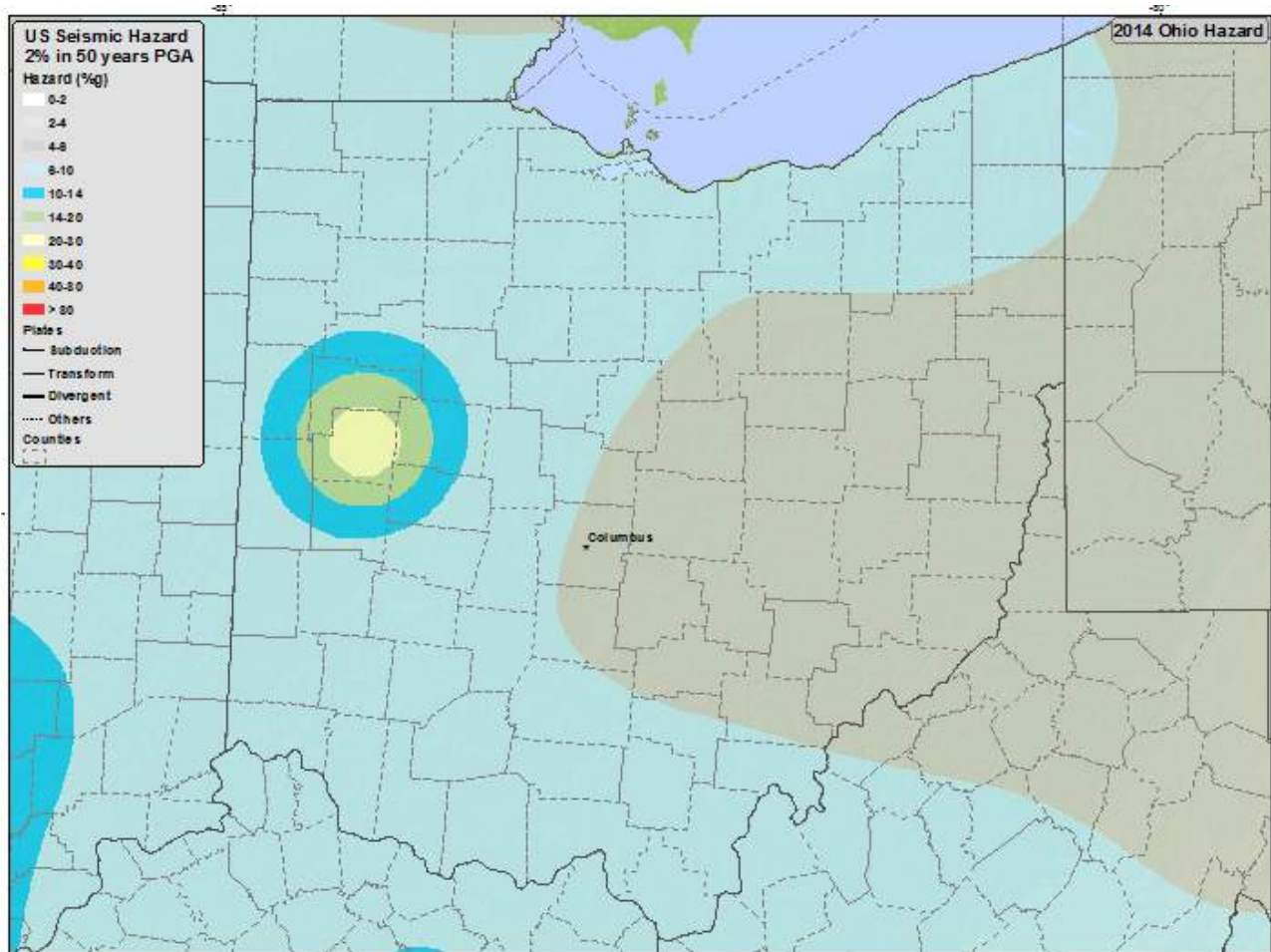
Figure 4.3.6: 2014 Seismic Hazard Map of state of Ohio
