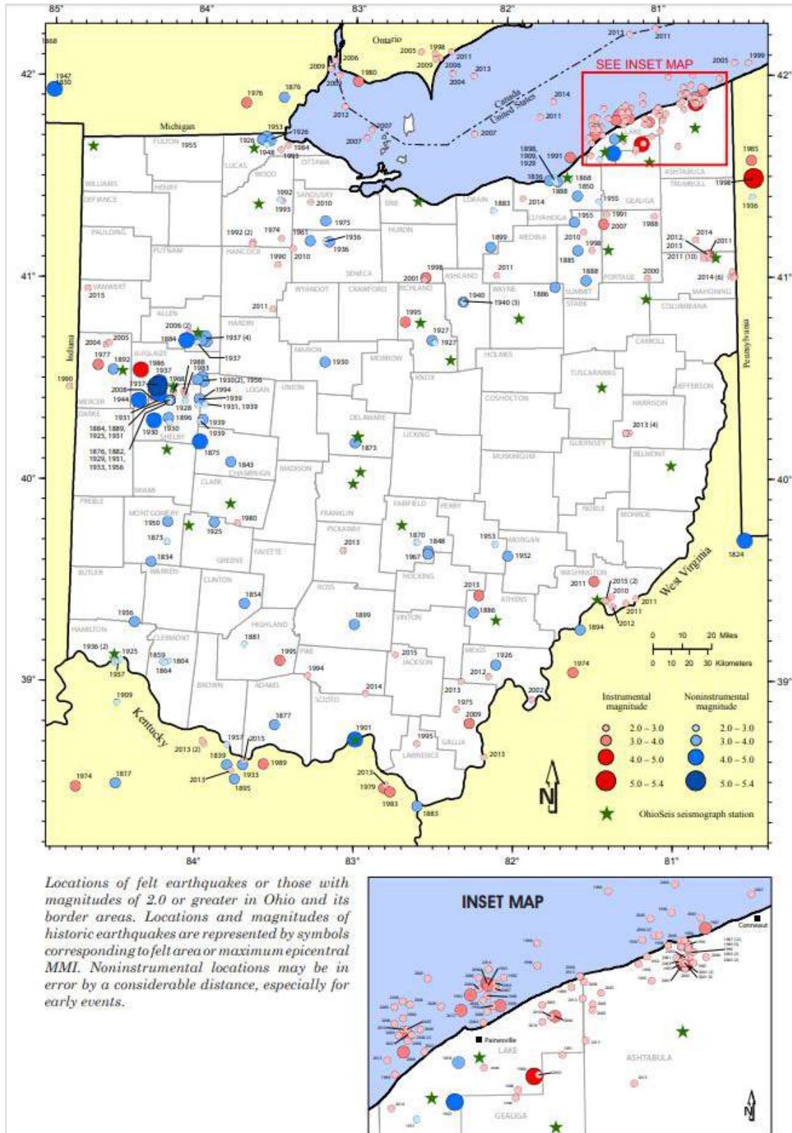
Figure 4.3.2: Earthquake Epicenters and Seismometers in Ohio
